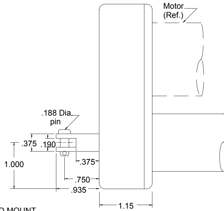
BUG END MOUNT EYE CLEVIS (.188)
