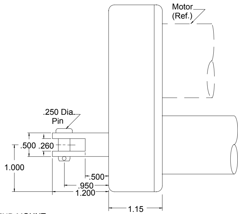
BUG END MOUNT EYE CLEVIS (.250)
