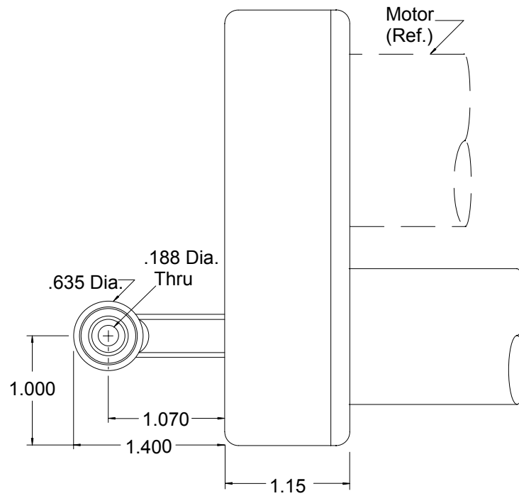
BUG END MOUNT ROD BEARING CLEVIS (.188)
