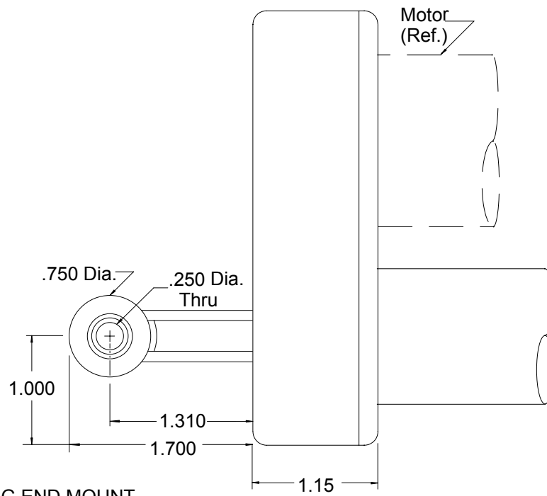
BUG END MOUNT ROD BEARING CLEVIS (.250)
