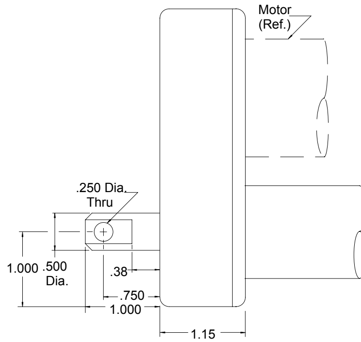
BUG END MOUNT ROD CLEVIS (.250)
