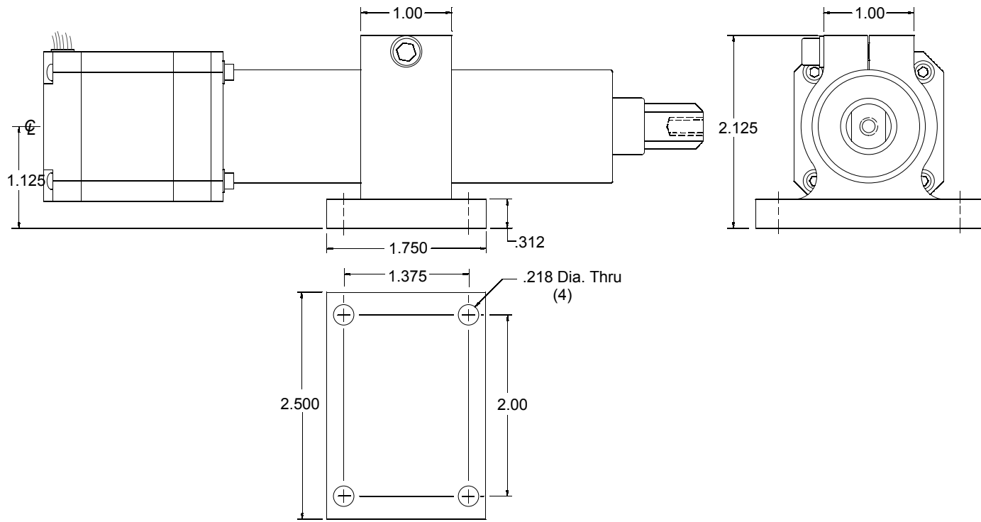
BLOCK MOUNT
