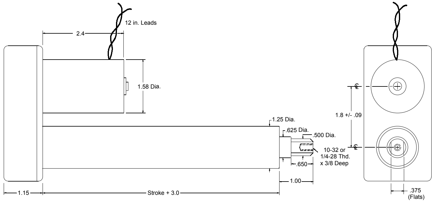
BUG (4 Inch Stroke) DC Motor
