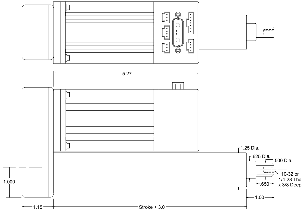
SMARTBUG (4 Inch Stroke) NEMA 23 Brushless Servo
