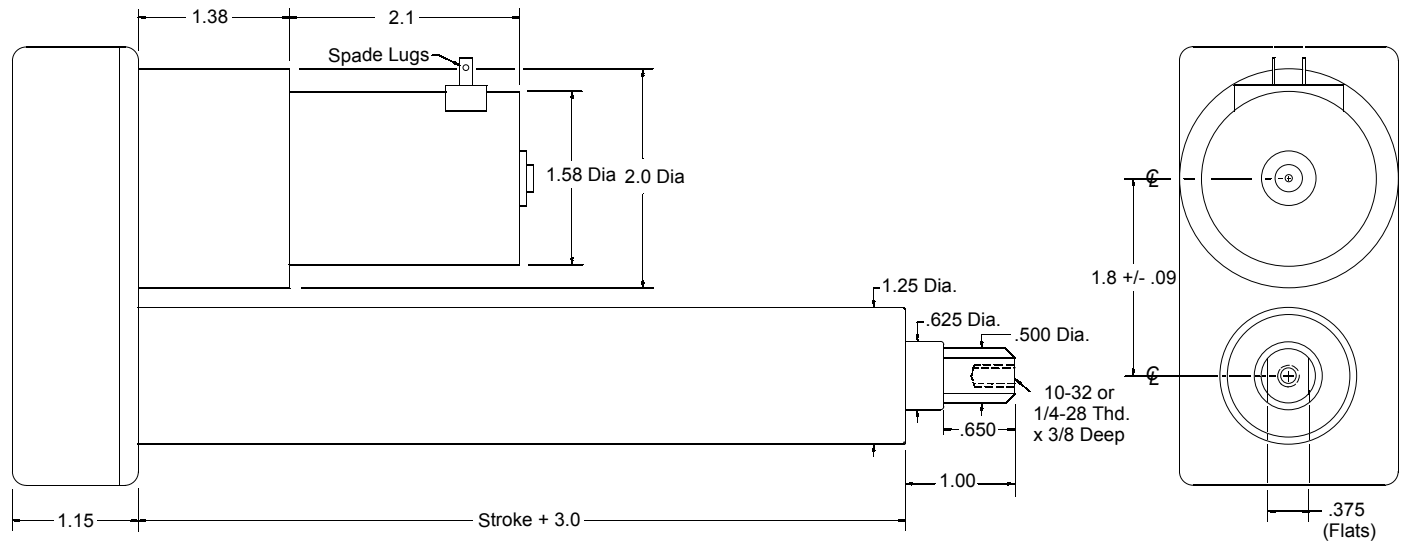
BUG (4 Inch Stroke) DC Gearmotor
