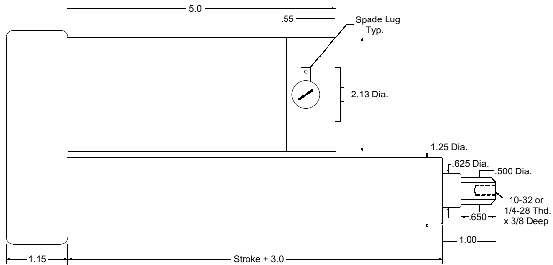
BUG (4 Inch Stroke) DC-146 Motor
