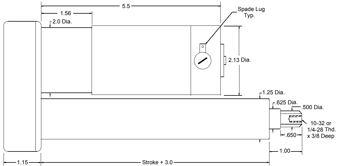
BUG (4 Inch Stroke) Large DC Gearmotor
