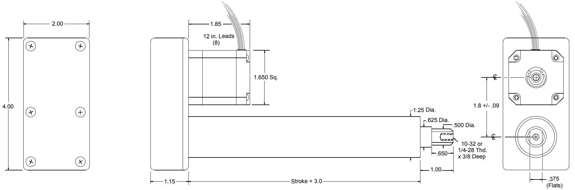
BUG (4 Inch Stroke) NEMA 17 Stepper Motor
