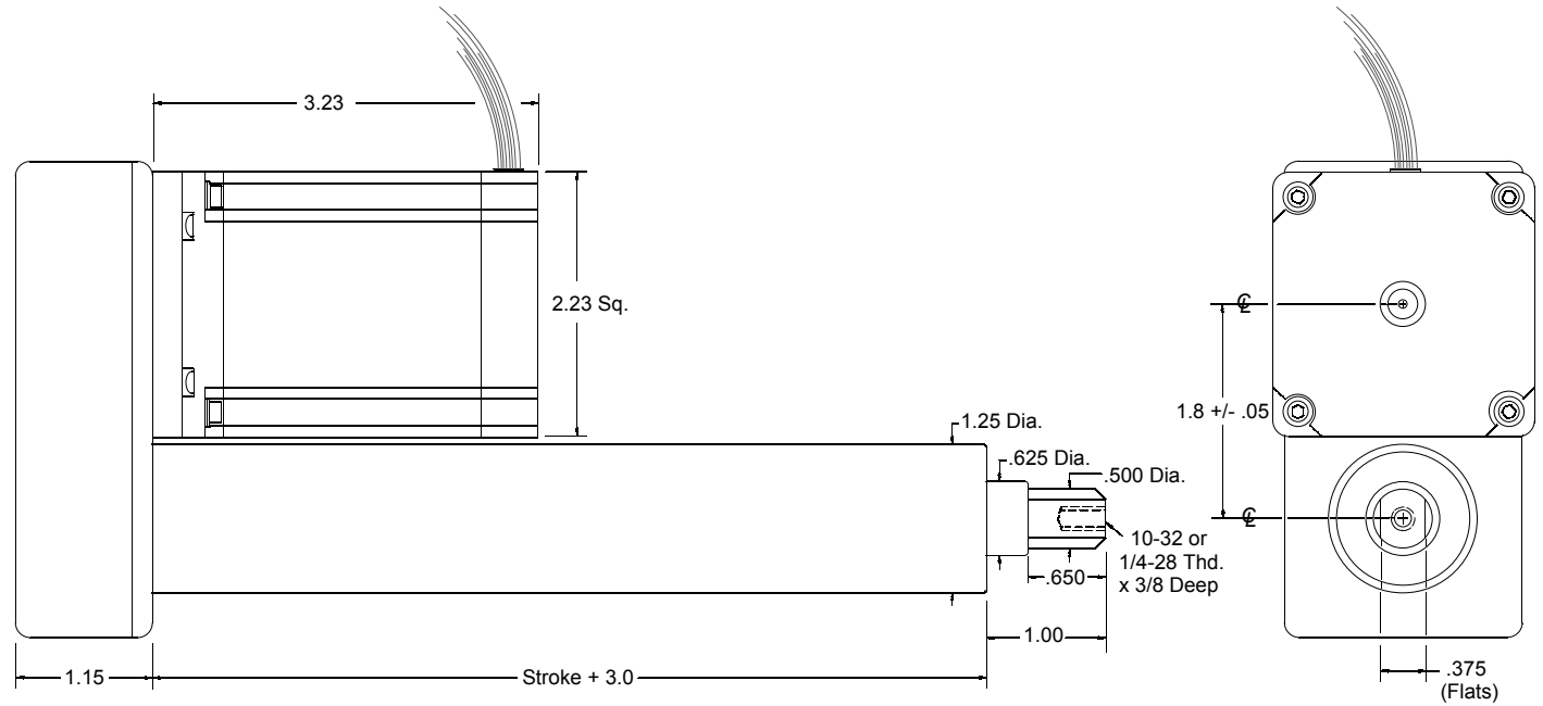
BUG (4 Inch Stroke) NEMA 23 Stepper Motor
