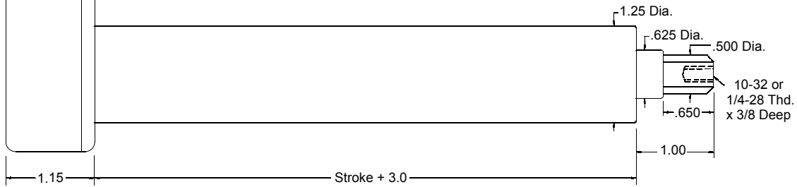
SMARTBUG (4 Inch Stroke) NEMA 17 Brushless Servo
