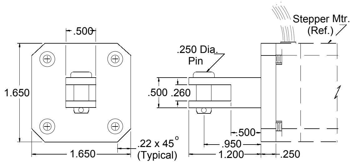
BASE EYE CLEVIS & MOUNTING PLATE .250 Dia.Pin (with cotter pin)
