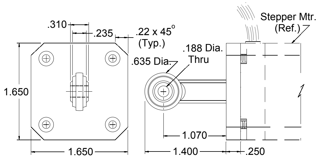
BASE ROD BEARING CLEVIS .188 Dia & MOUNTING PLATE
