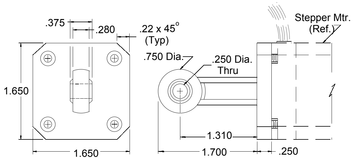
BASE ROD BEARING CLEVIS .250 Dia & MOUNTING PLATE
