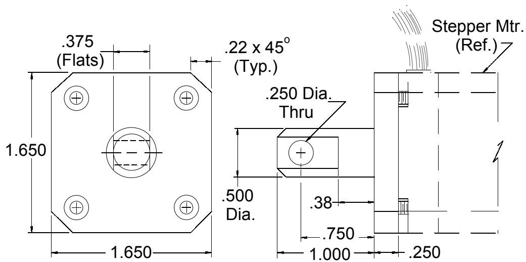
BASE ROD CLEVIS & MOUNTING PLATE
