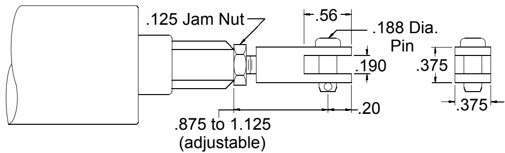
NOSE EYE CLEVIS - .188 PIN (with cotter pin)
