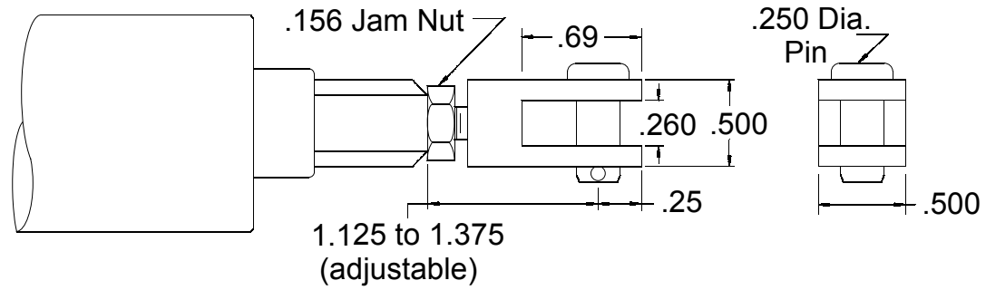
NOSE EYE CLEVIS - .250 Pin (with cotter pin)
