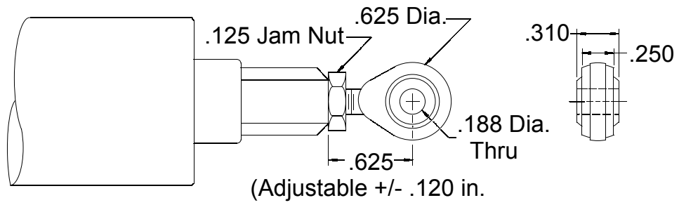
NOSE ROD BEARING CLEVIS - .188 ID
