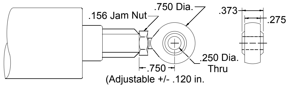
NOSE ROD BEARING CLEVIS - .250 ID
