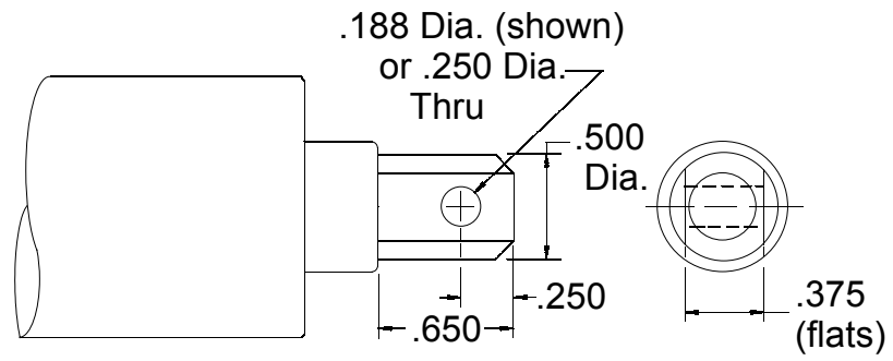
NOSE ROD CLEVIS -.188/.250 Dia
